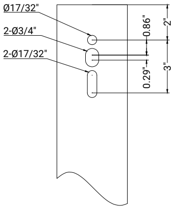
Pre-drilled measurements
