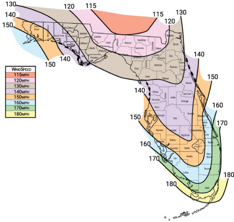
FBC 2023 / ASCE 7-10 WIND MAP EPA LOAD RATING - ULTIMATE 3 SECOND GUST WIND
